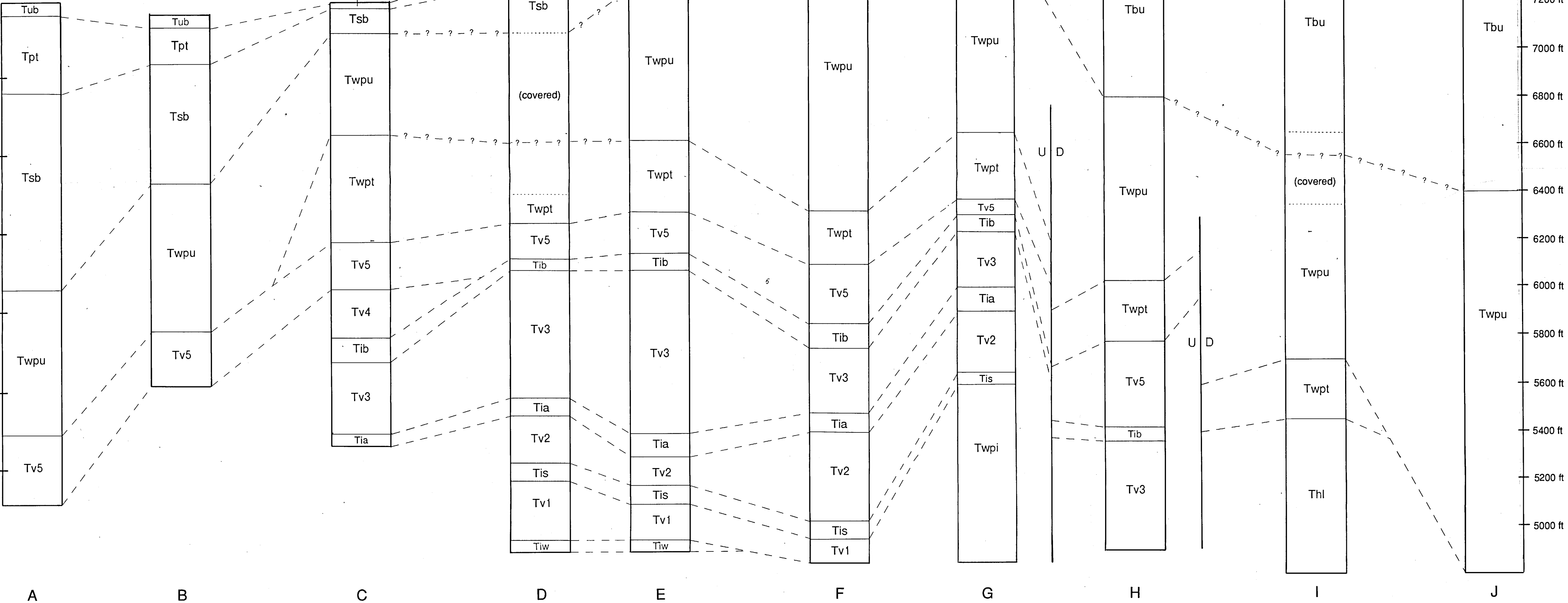
Stratigraphy of the West Side of Hart Mountain, Southern Oregon
