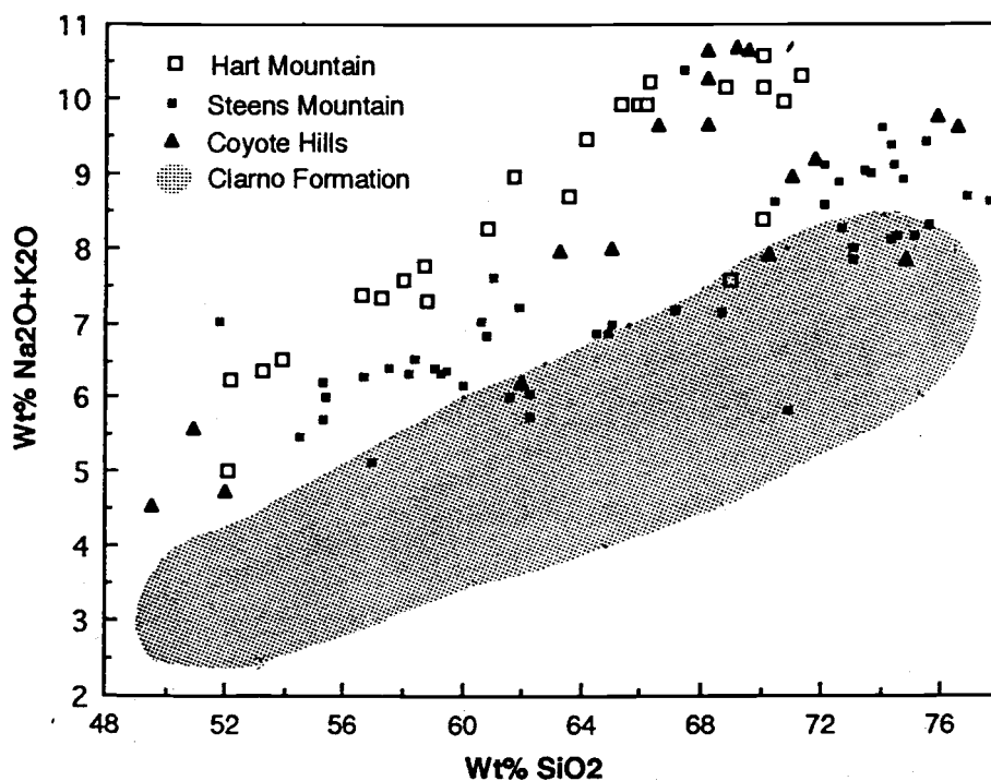
Figure 4: Plot of weight percent Na 2 O+K 2 O versus weight percent SiO 2 for volcanic rocks older than Steens Basalt in eastern Oregon. Data compiled from: Steens Mountain: Langer (1991), Carlson and Hart (1987), Harrold (1973), and Fuller (1931); Coyote Hills: Thomas (1981). The field for the Clarno Formation is from Rogers and Novitsky-Evans (1977), Noblett (1981), Mullen (1978), and Oles and Enlows (1972).
